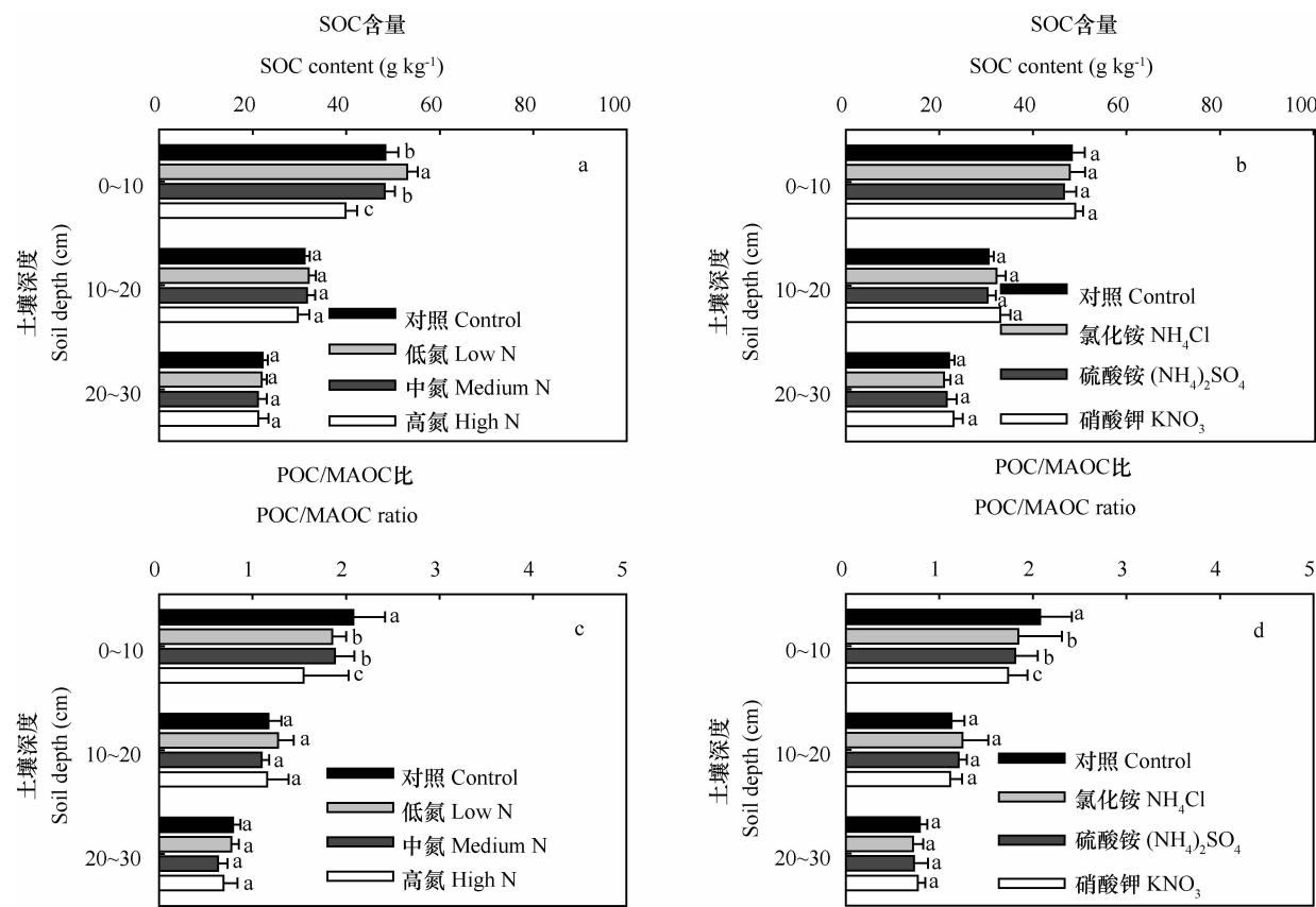
图 2 不同施氮剂量和施氮类型下总 SOC 含量和 POC/MAOC 比值的变化 (图中不同字母表示同层土壤不同处理差异显著) Fig. 2 Variation of total SOC content and POC/MAOC ratio relative to rate and form of N applied (In the figure, different letters indicate significant difference between treatments within the same depth soil layer)
