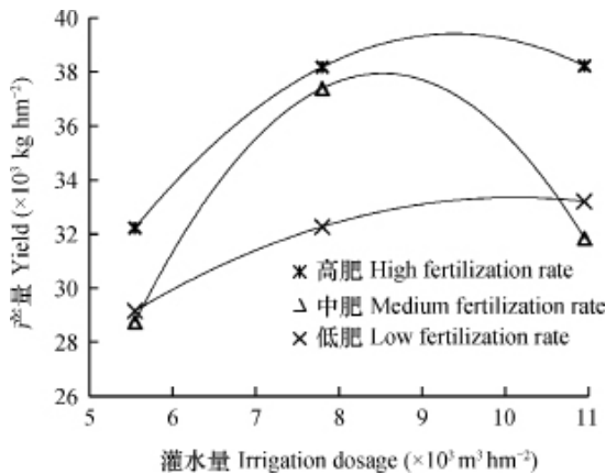
注：高肥、中肥、低肥的施肥量分别为750 kg hm -2 、450 kg hm -2 和300 kg hm -2 Note: The high, medium and low fertilization rate was 750 kg hm -2 , 450 kg hm -2 and 300 kg hm -2 , respectively
