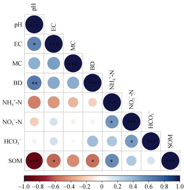
图 2 土壤理化性质间的 Spearman 相关性 Fig. 2 The Spearman correlations between soil physiochemical properties
