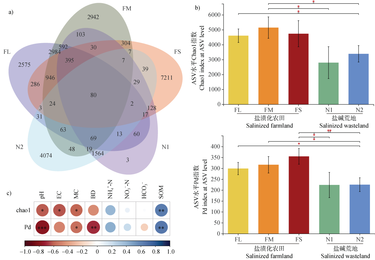
注：韦恩图代表不同盐渍化土壤共有和特有的原核生物 ASVs (a)。不同盐渍化土壤原核生物 α 多样性指数及其差异显著性 (b)。土壤原核生物 α 多样性与土壤理化性质间的 Spearman 相关(c)。Note: The Venn diagram represents the number of shared and specific ASVs across different saline soils (a). The significance of α-diversity indexes in difference saline soils (b). The Spearman correlations between soil prokaryotic α-diversity and soil physicochemical properties (c).
