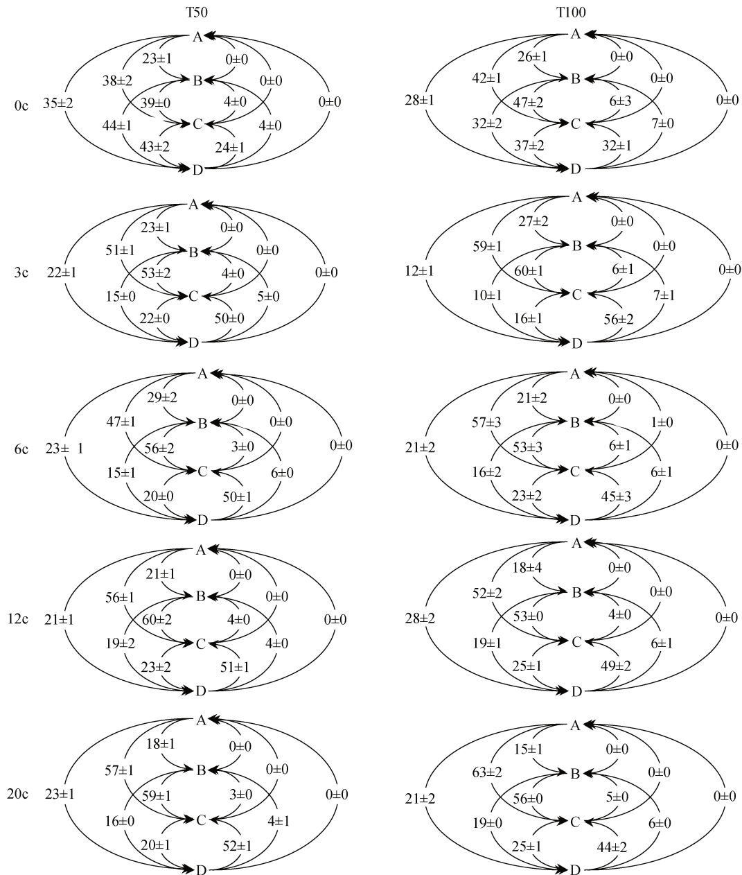
注：A, B, C 和 D 分别代表 5~2 mm, 2~0.25 mm, 0.25~0.053 mm 和 <0.053 mm 团聚体。Note: A, B, C, and D represent 5-2 mm, 2-0.25 mm, 0.25-0.053 mm and < 0.053 mm aggregates.
