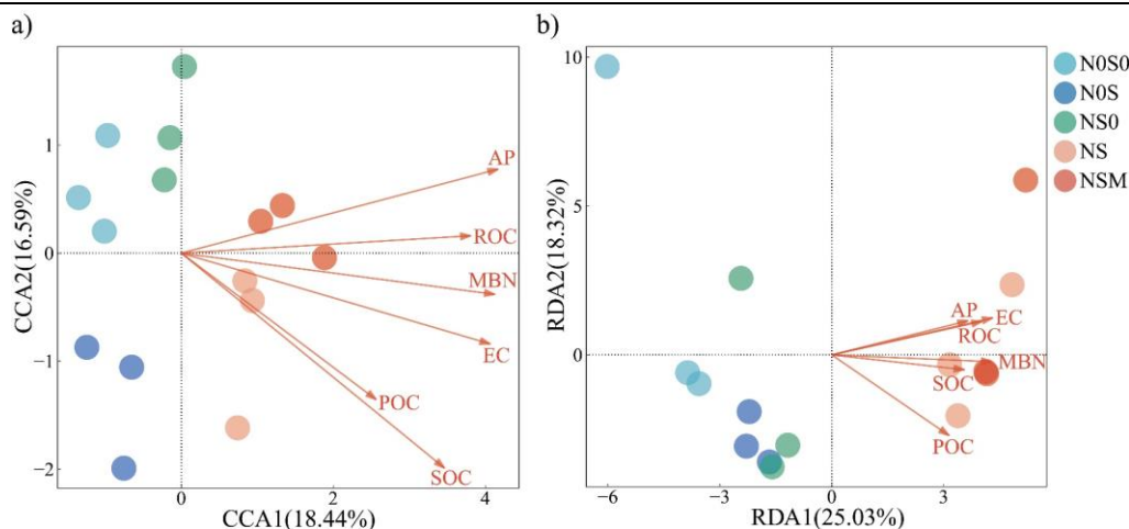
注：(a) 土壤细菌群落组成和理化性质的典范对应分析 (CCA)；(b) 土壤真菌群落组成和理化性质的冗余分析 (RDA)。 Note: (a) Canonical correspondence analysis (CCA) of soil bacterial community composition and physicochemical properties; (b) Redundancy analysis (RDA) of soil fungal community composition and physicochemical properties.
