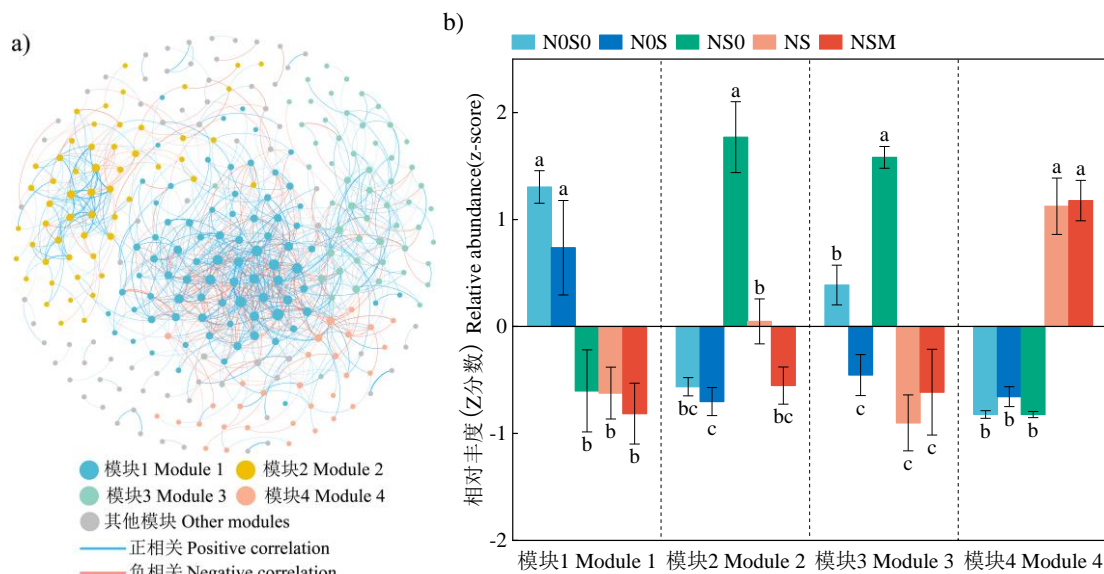
注：网络中的 OTUs 相对丰度高于总丰度的 0.05%，且 OTUs 间具有强相关性（Spearman 相关系数值 (r) \geq 0.7 ，校正后的 P < 0.01 ）。蓝线表示正相关关系，红线表示负相关关系，线条越粗表示 Spearman 相关系数值 (r) 越大，节点的大小按度（即与该节点连接的边的数量的多少）的大小赋值，连接的边越多，节点越大。Note: The relative abundance of OTUs in the bacterial-fungal co-occurrence network was higher than 0.05% of the total relative abundance, and there was a strong correlation between OTUs (Spearman's r \geq 0.7 , FDR-adjusted P < 0.01 ). The blue line represents the positive correlation, while the red line represents the negative correlation. The thicker line indicates the larger Spearman correlation value (r) , the size of the node is assigned according to the size of the degree (that is, the number of edges connected to the node), and the more connected edges, the larger the node.
