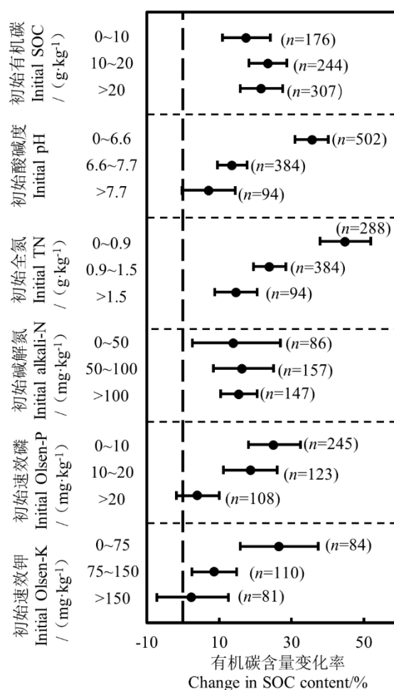
图 2 不同初始土壤理化性质下长期种植作物土壤有机碳含量变化率 Fig.2 Changes in SOC contents under different initial properties of soil
