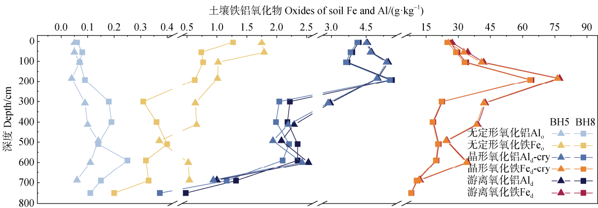
图 8 BH5 和 BH8 钻孔点红壤风化壳铁铝氧化物含量（以单质 Fe 和单质 Al 的形式表征含量）的深度变化特征 Fig. 8 Changes of Fe and Al oxide contents (expressed in the forms of elemental Fe or Al) of red soil regolith samples with depth in boreholes BH5 and BH8
