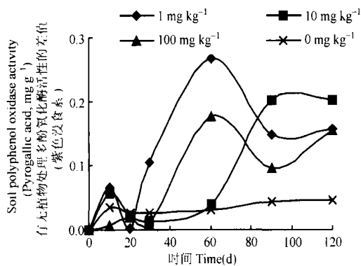
图 2 黑麦草对苯并[a]芘污染土壤中多酚氧化酶活性差值动态的影响 Fig 2 Effect of ryegrass on polyphenol oxidase activities* in B[a]P-contaminated soil
