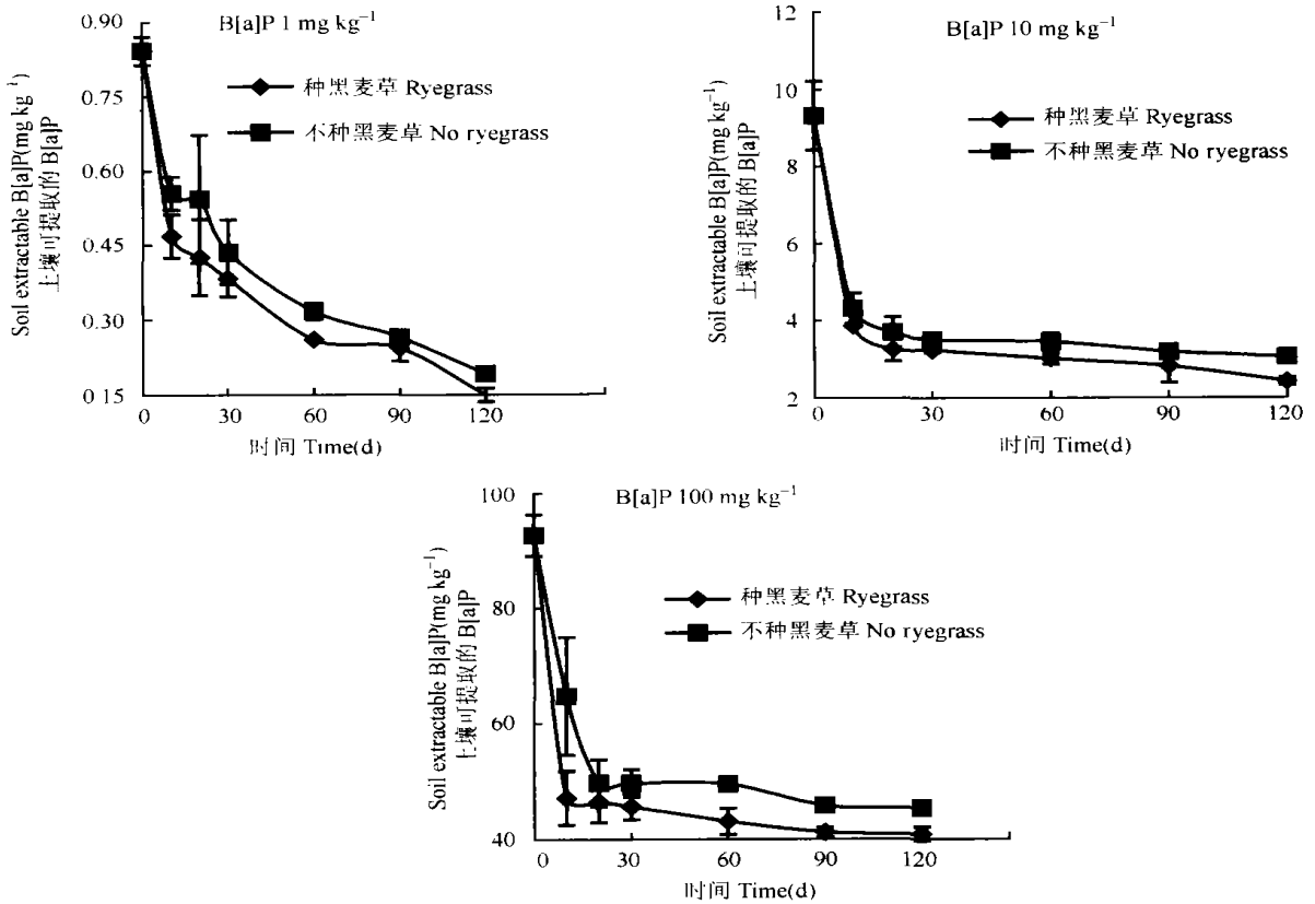
图 1 黑麦草对污染土壤中可提取态苯并[a]芘浓度动态变化的影响 Fig 1 Dynamics in extractable B[a]P in soil with and without growth of ryegrass plants
