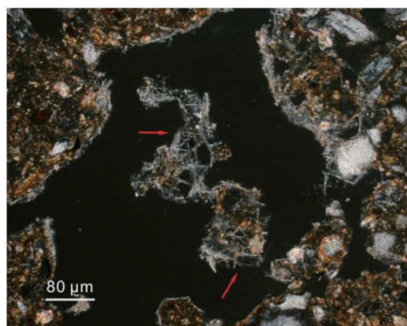
c Ah 1 /Ap 3 层中针状方解石 (正交偏光 20×10) c Needleshaped secondary-calcite in Ah 1 /Ap 3 horizon (crossed polarised light 20×10)
