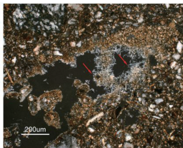
d Ah 2 /Ap 4 层中针状方解石 (正交偏光 10×10) d Needleshaped secondary-calcite in Ah 2 /Ap 4 horizon (crossed polarised light 20×10)
