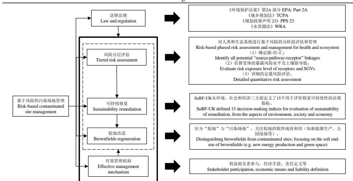
EPA: Part 2A: Environmental Protection Act 1990: Part 2A; TCPA: Town and Country Planning Act; PPS 23: Planning Policy Statement 23; WRA: Water Resources Act; SGVs: Soil Guideline Values; SuRF-UK: Sustainable Remediation Forum UK
