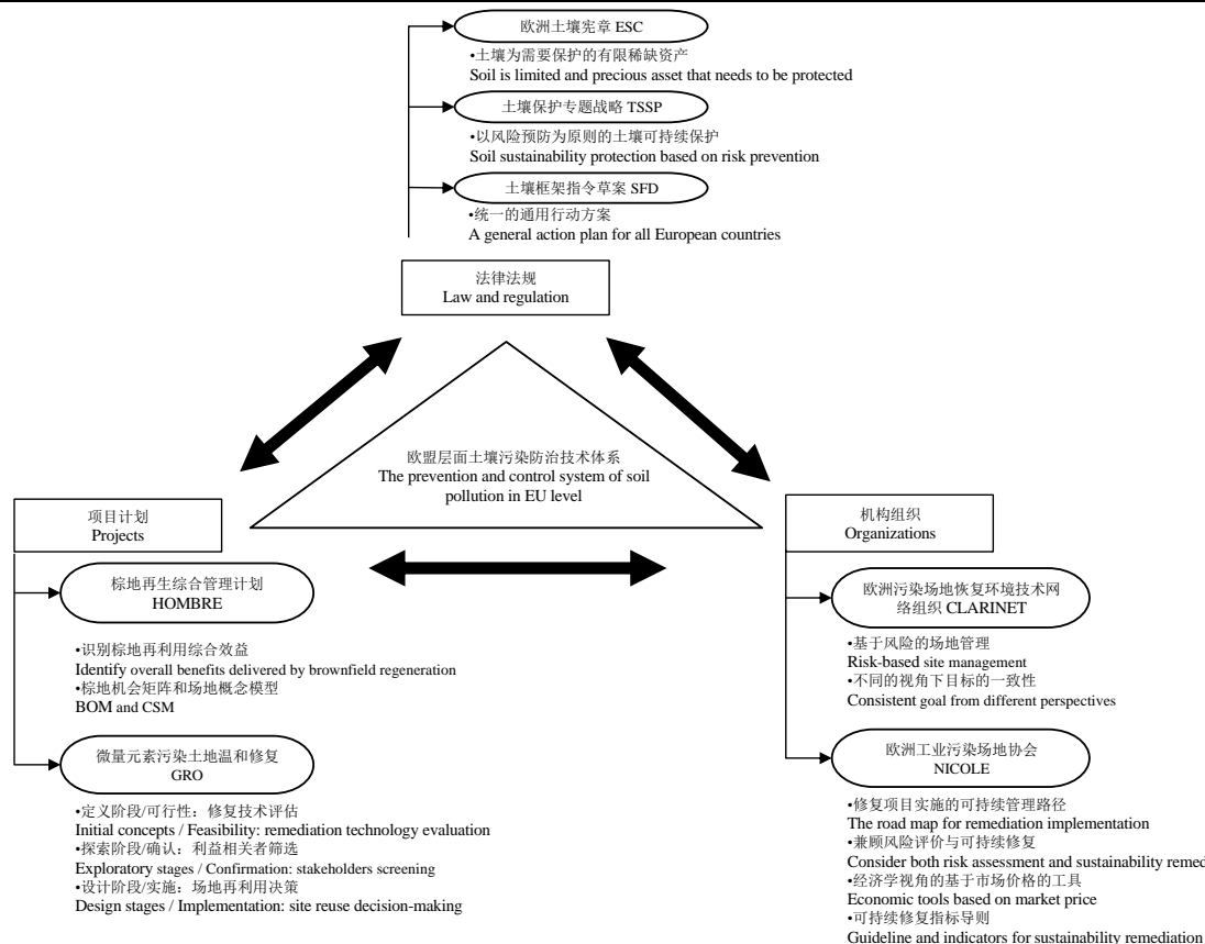
ESC: European Soil Charter; TSSP: Thematic Strategy for Soil Protection; SFD: Soil Framework Directive; HOMBRE: Holistic Management of Brownfield Regeneration; GRO: Gentle remediation options; CLARINET: The Contaminated Land Rehabilitation Network For Environmental Technologies in Europe; NICOLE: Network for Industrially Contaminated Land in Europe; BOM: Brownfield Opportunity Matrix; CSM: Conceptual site model
