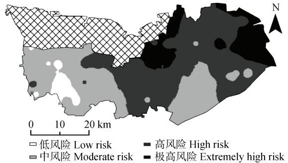
注：低风险 CR'<0.1，中风险 CR'0.1~0.3，高风险 CR'0.3~0.5，极高风险合计 CR'>0.5。Note: Low risk CR'<0.1; Moderate risk CR'0.1~0.3; High risk CR'0.3~0.5; Extremely high risk CR'>0.5.
