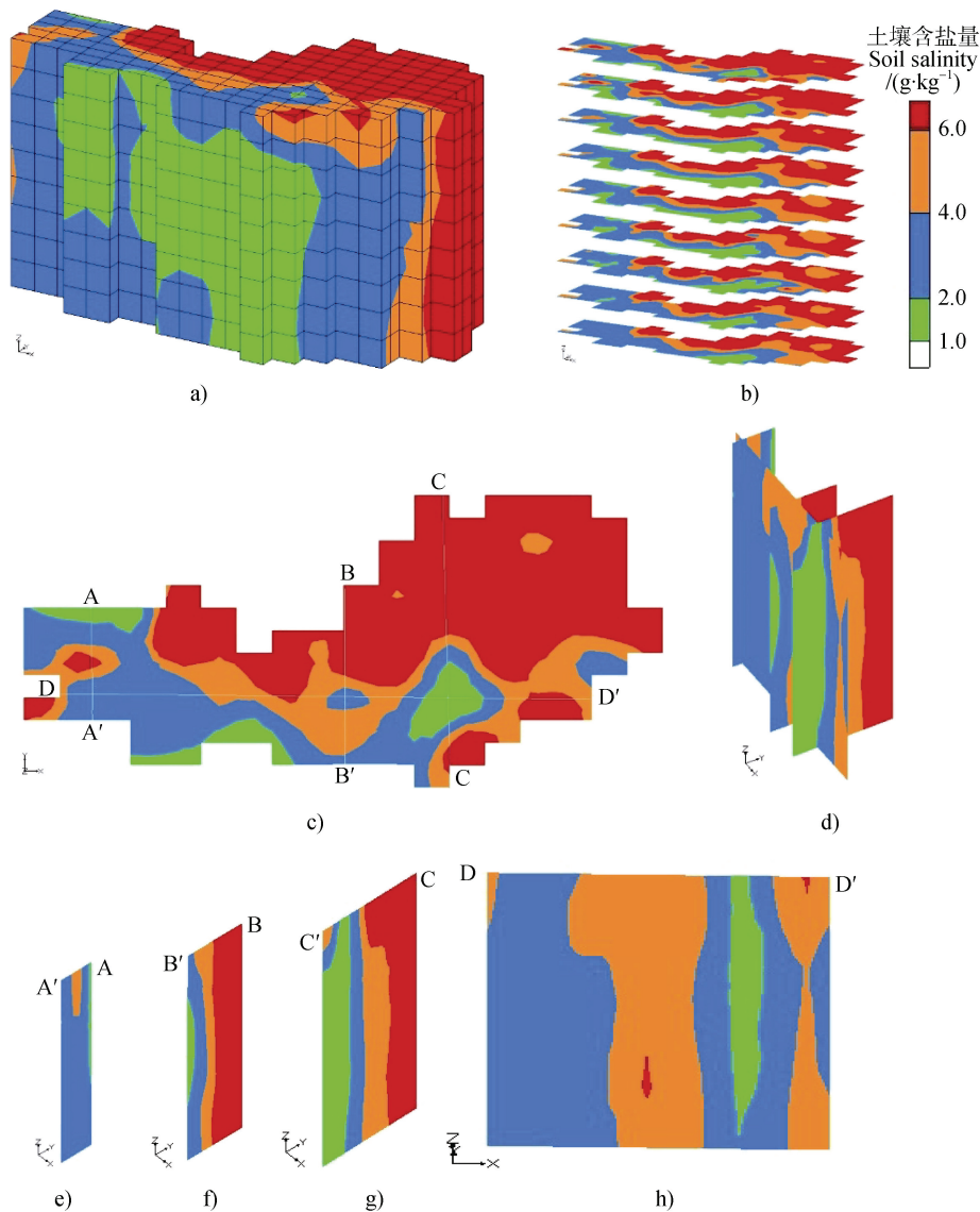
注: a)土壤盐分三维分布(0~52.5cm), b)各层土壤盐分分布, c)~h)典型截面土壤盐分三维空间分布。Note: a)Three-dimensional distribution of soil salt (0~52.5cm), b)Distribution of soil salt in each layer, c)~h)Three-dimensional distribution of soil salt in typical sections.
