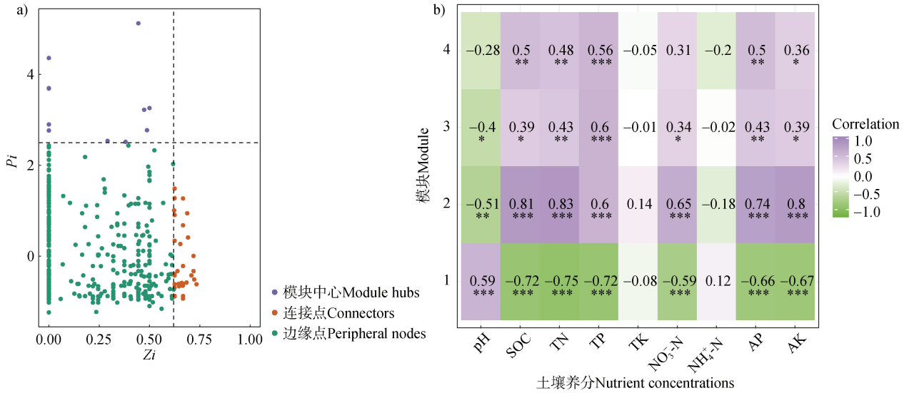
注：a) 为 Zi-Pi 图；b) 为模块累计丰度与土壤养分指标相关性分析；色柱表示相关性，绿色表示负相关，紫色表示正相关，*表示 P < 0.05 ，**表示 P < 0.01 ，***表示 P < 0.001 。Note: a) was Zi-Pi plot; b) was correlation analysis between the cumulative abundance of modules and soil nutrient concentrations; The color column indicated correlation, green indicated negative correlation, and purple indicated positive correlation, *indicated P < 0.05 , **indicated P < 0.01 , ***indicated P < 0.001 .
