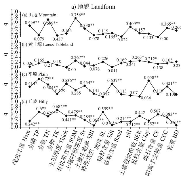
Fig. 3 Statistics of the explanatory power (q value) of soil quality influencing factors on soil quality
